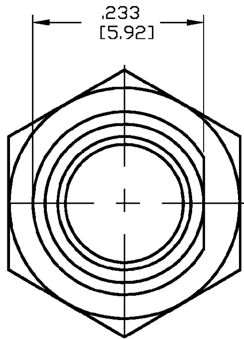
VIEW SHOWN WITHOUT HEX NUT & LOCKWASHER
